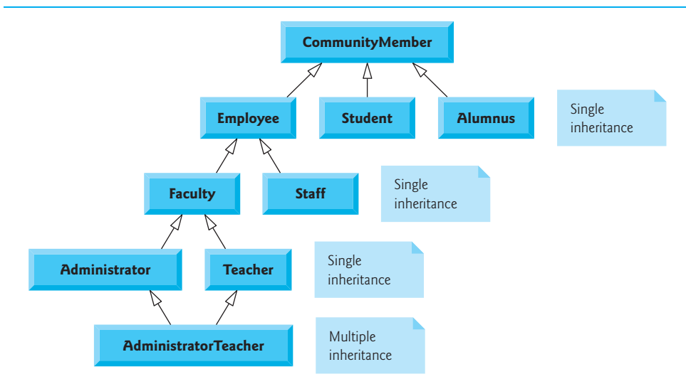
Fig. 20.2 | Inheritance hierarchy for university CommunityMembers .
